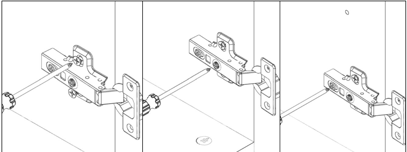
HEIGHT ADJUSTMENT
